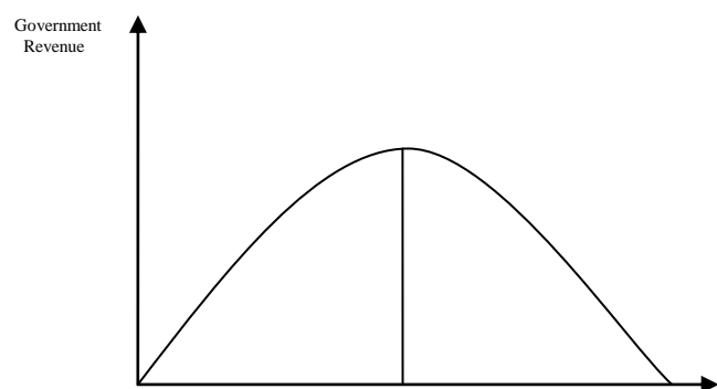
Figure 1: Laffer curve
