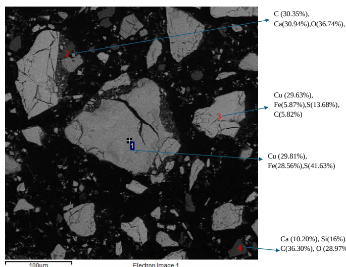
Fig.1: SEM results of Chalcopyrite
